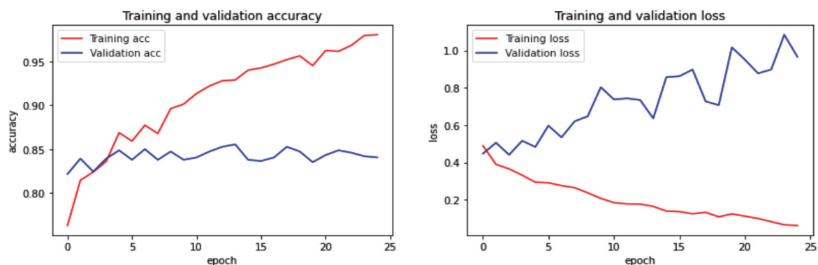
Figure 8. This figure shows the accuracy and loss analysis of visual geographical group convolutional neural network.
