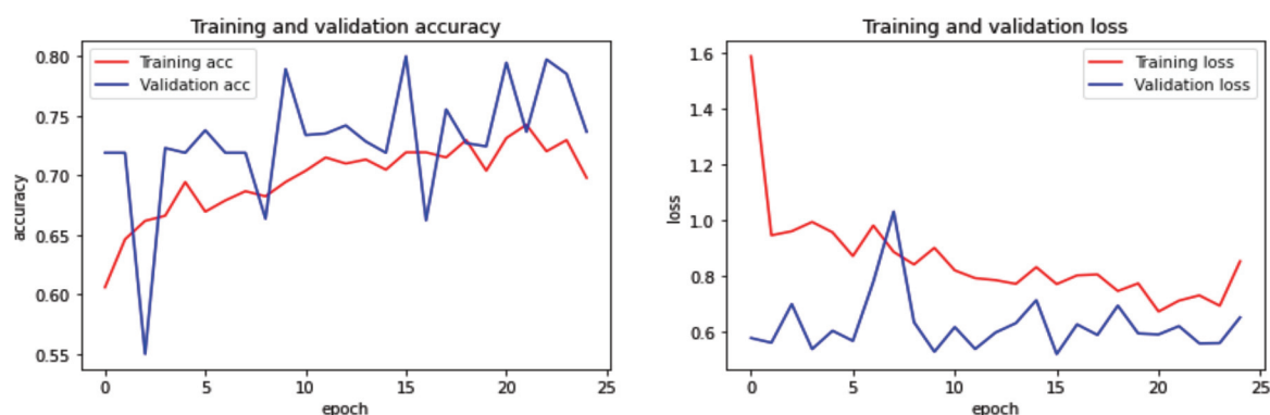
Figure 10. This figure shows the accuracy and loss analysis of residual convolutional neural network. acc: Accuracy
