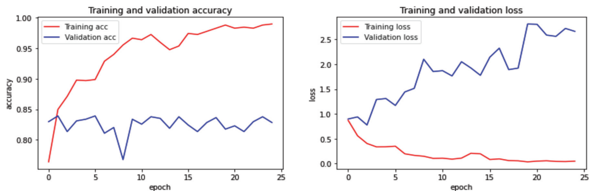
Figure 9. This figure shows the accuracy and loss analysis of google convolutional neural network.
