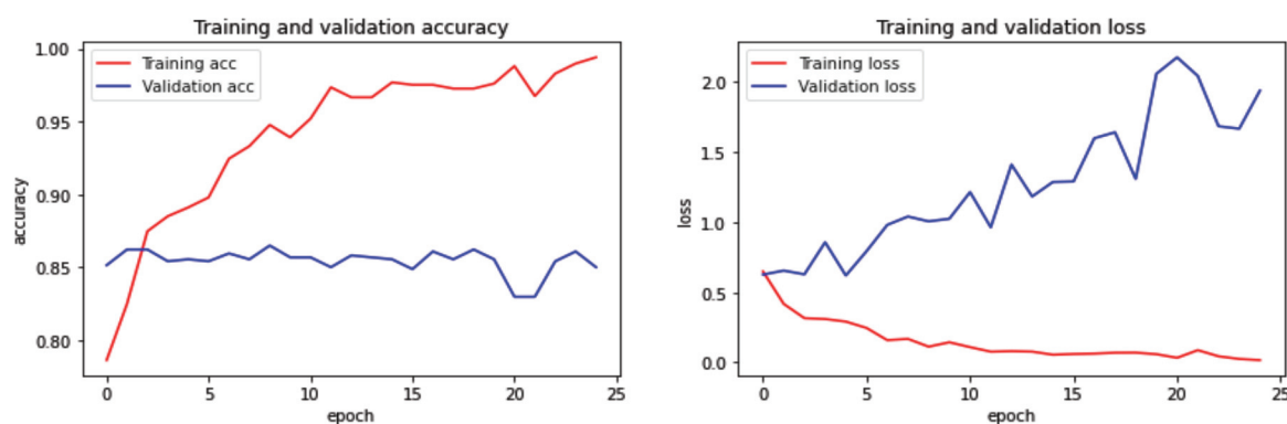
Figure 12. This figure shows the accuracy and Loss analysis of the proposed ensemble framework for breast cancer prediction.
