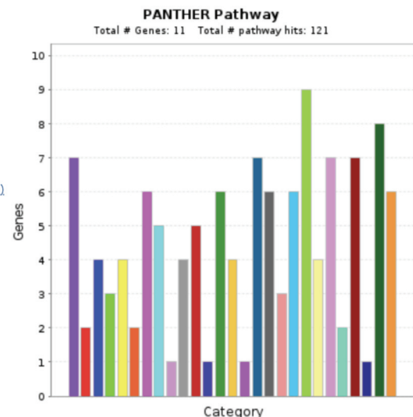
Figure 2. This figure shows the molecular pathway in which PIK3CA interacting proteins are involved. PIK3CA : Phosphatidylinositol 3-kinase
